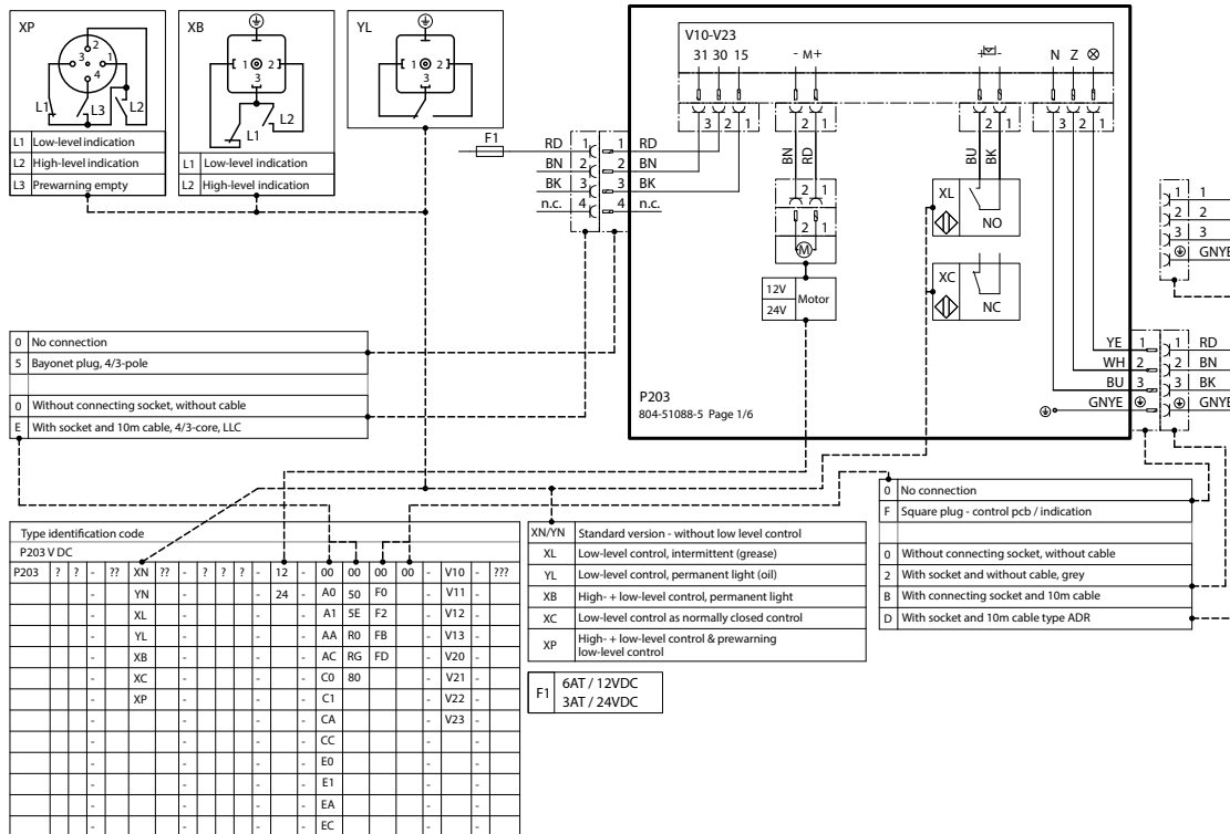
Connection diagram P203 V DC with control PCB V Fig. 43
