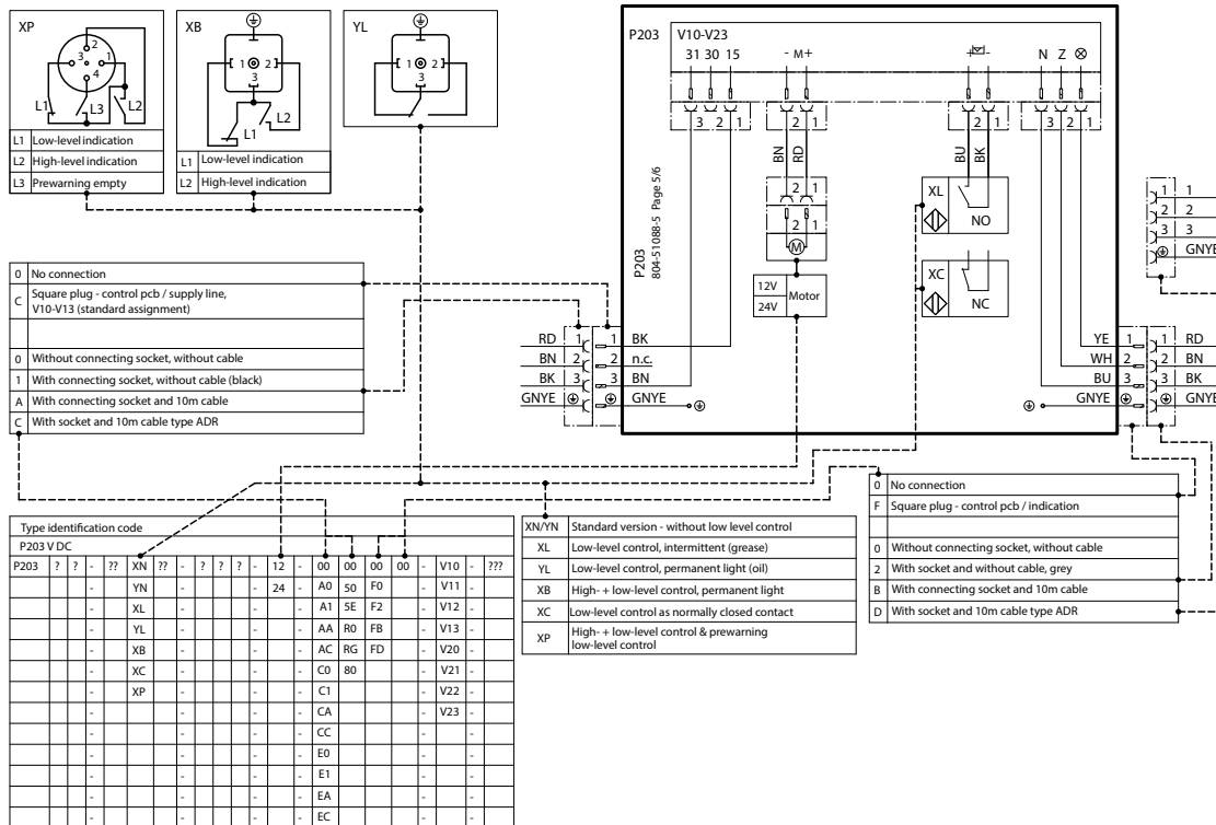
Connection diagram P203 V DC with control PCB V Fig. 47
