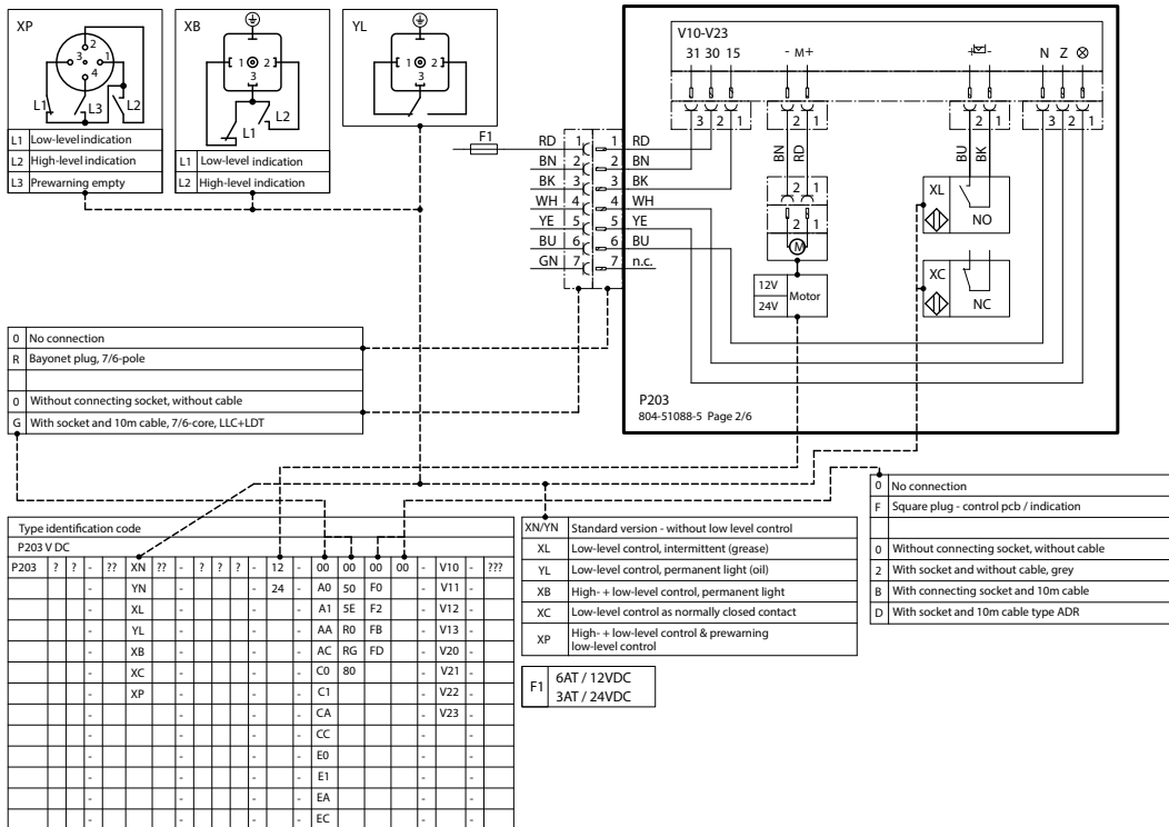
Connection diagram P203 V DC with control PCB V Fig. 44
