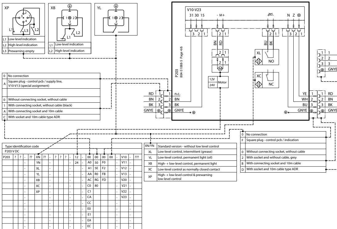
Connection diagram P203 V DC with control PCB V Fig. 46
