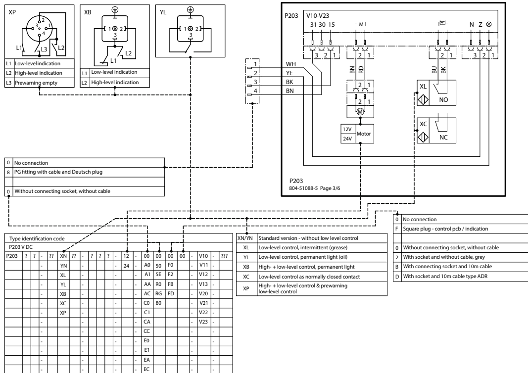
Connection diagram P203 V DC with control PCB V Fig. 45
