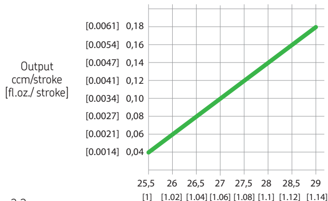
Adjusting the output volume on pump element R Fig. 11
